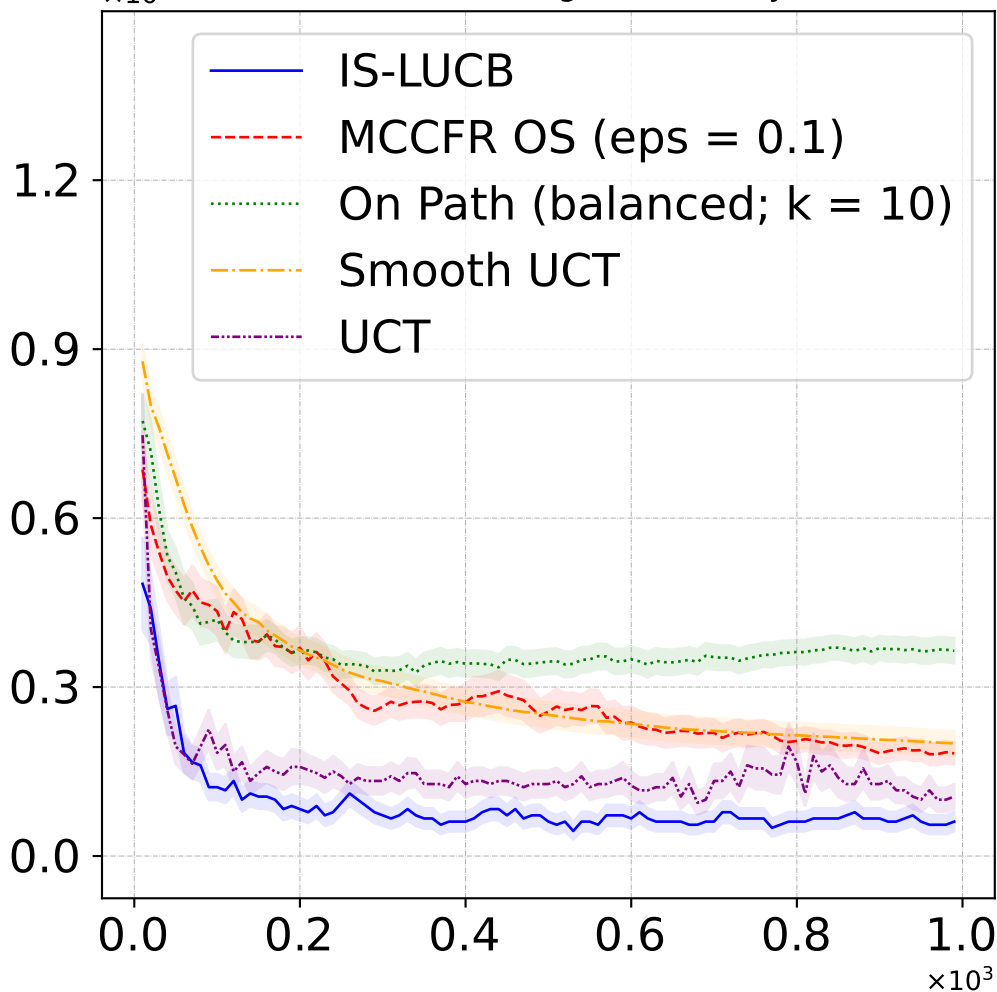
\times 10^{-1} Kuhn Poker, Best Algorithms, Player x
